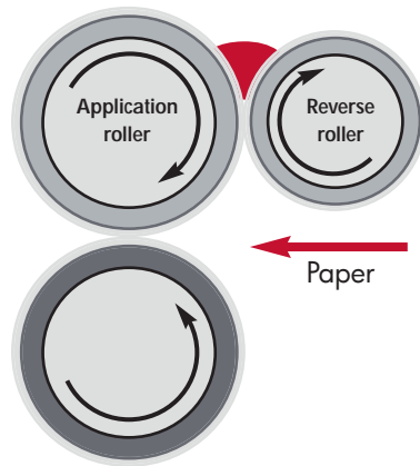
Figure 1: The HP Indigo UV Coater coating head Two separate rollers optimise process control and results.
